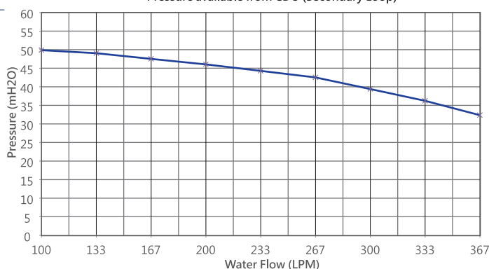
TC368 / TC368S Pressure available from CDU (Secondary Loop)
